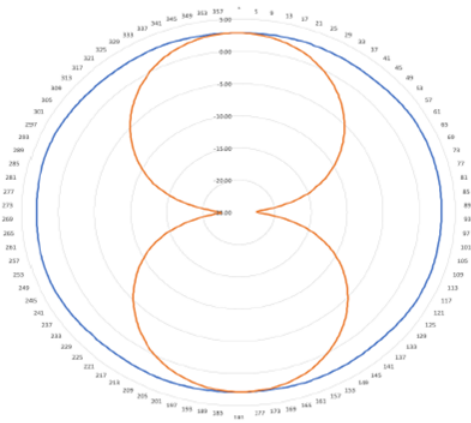
2.4 GHz Antenna Radiation Pattern
