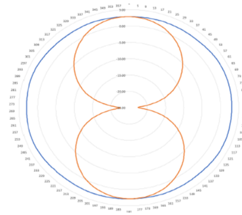
5.5 GHz Antenna Radiation Pattern
